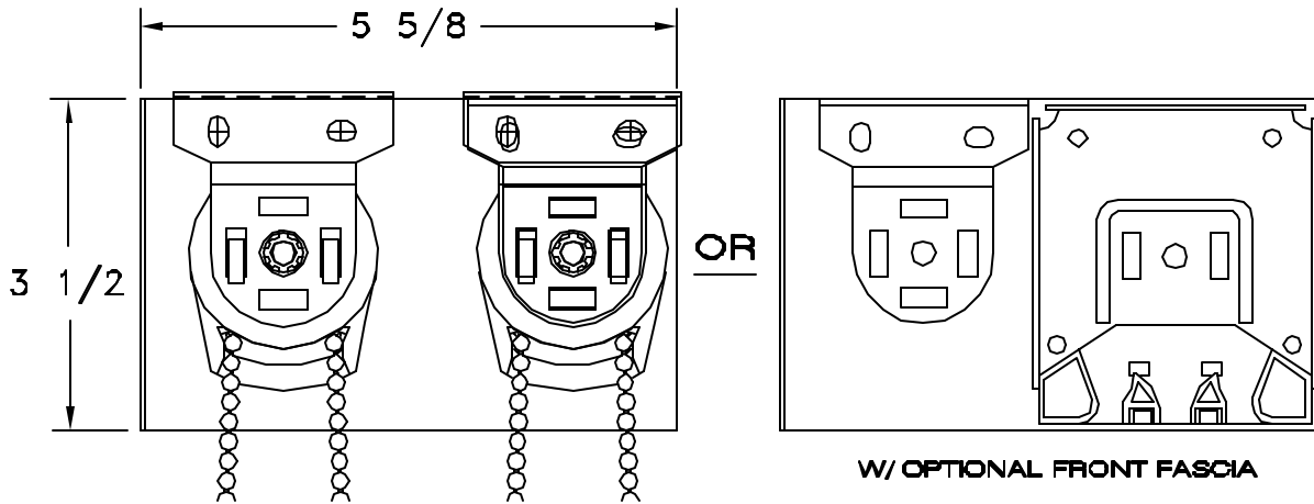
TANDEM-WALL MOUNT BRACKET ASSEMBLY
