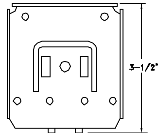
3" IDLER W/DIVERTER
